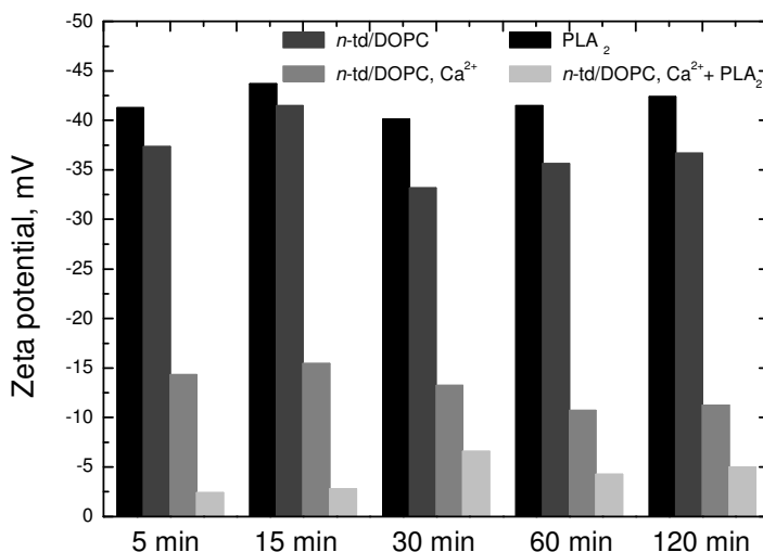
Fig. 15. Zeta potential of n -tetradecane droplets with DOPC (and \text{Ca}^{2+} ) or in the presence of \text{PLA}_2 at 37^\circ\text{C} as a function of time at pH 8.
