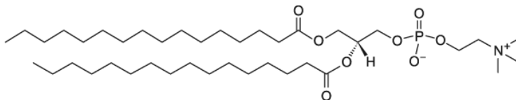
Fig. 1. Molecular structure of DPPC (1,2-dipalmitoyl- sn -glycero-3-phosphocholine).
