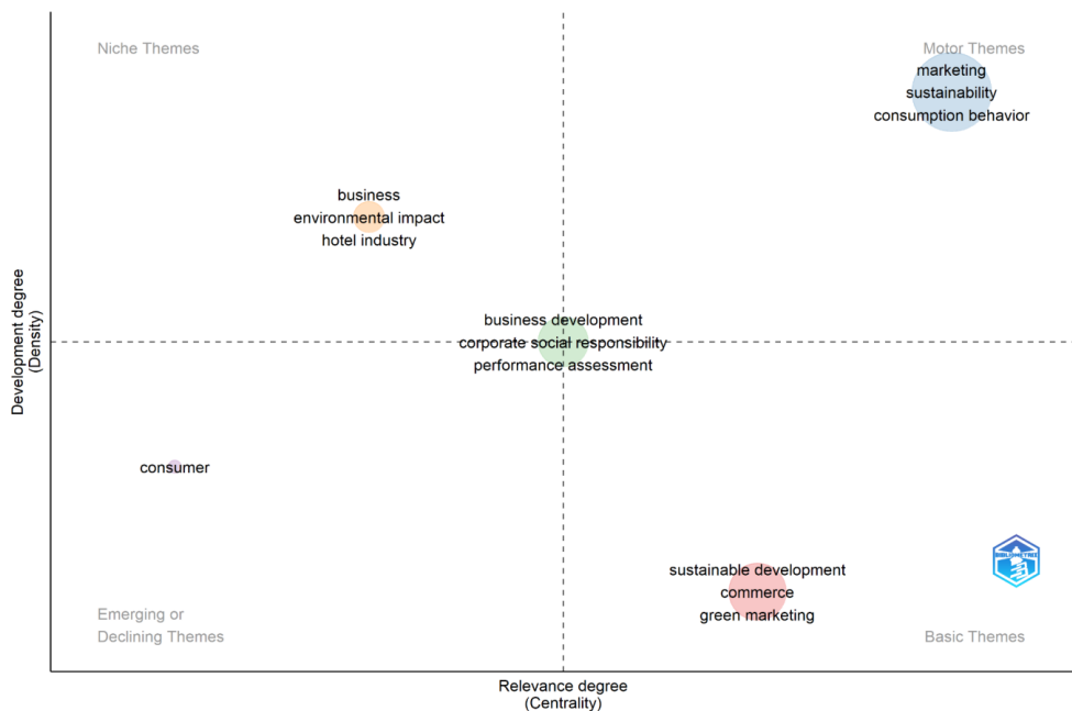
Figure 4. Thematic map
