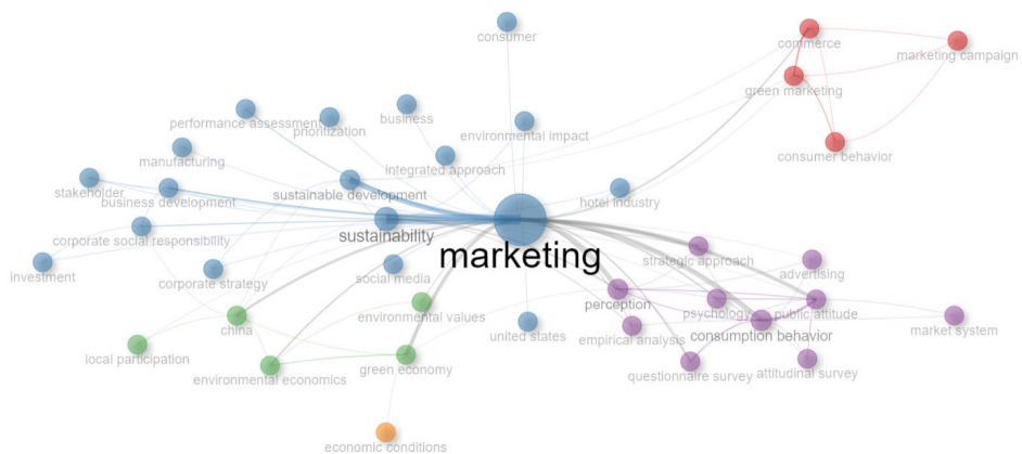
Figure 7. Co-occurrence network
