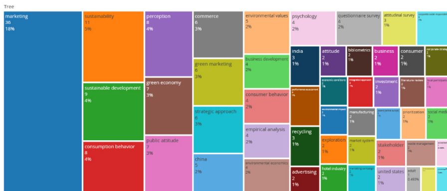
Figure 5. Tree map
