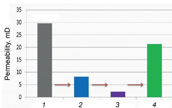
Fig. 10. Change in the absolute permeability of the model (anhydrous sample) (1) during the simulation of residual water saturation (2), clogging with technical water (3) and the effect on the model of the “Emir” composite (4)
