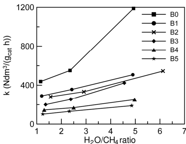
Fig. 2. The rate constant as a function of the reagents \text{H}_2\text{O}:\text{CH}_4 ratio at the temperature 550°C and at the constant amount (4%) of \text{H}_2 in the reaction mixture.
