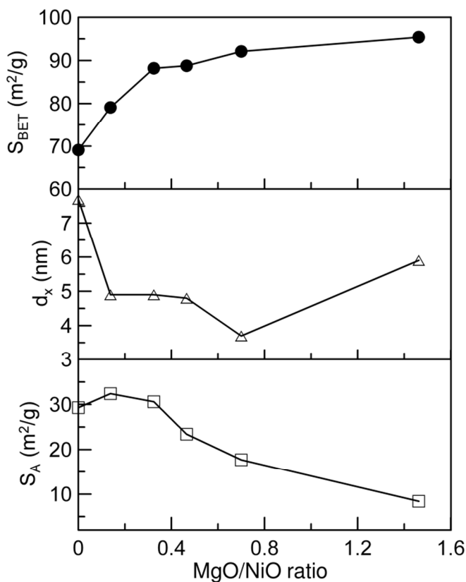
Fig. 1. Changes of the total S_{\text{BET}} and active S_A surface areas and the mean size of nickel crystallites d_x as a function of the MgO/NiO ratio after reduction at 800°C.
