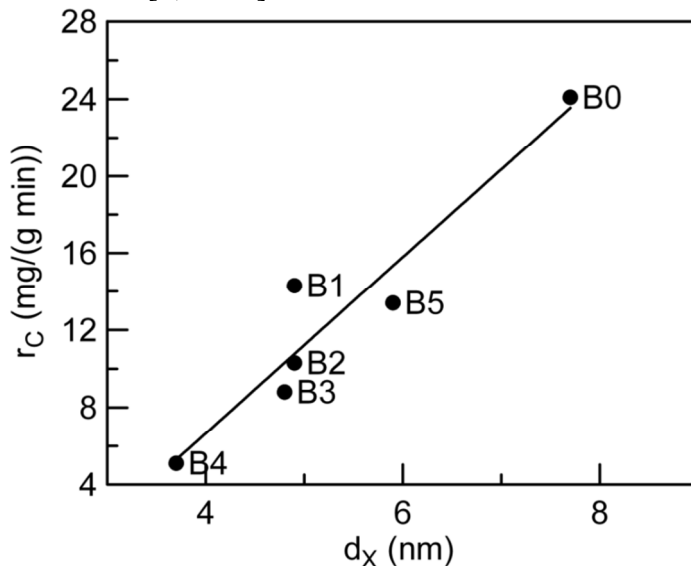
Fig. 12. The coking rate as a function of the mean sizes of nickel crystallites for the catalysts studied.
