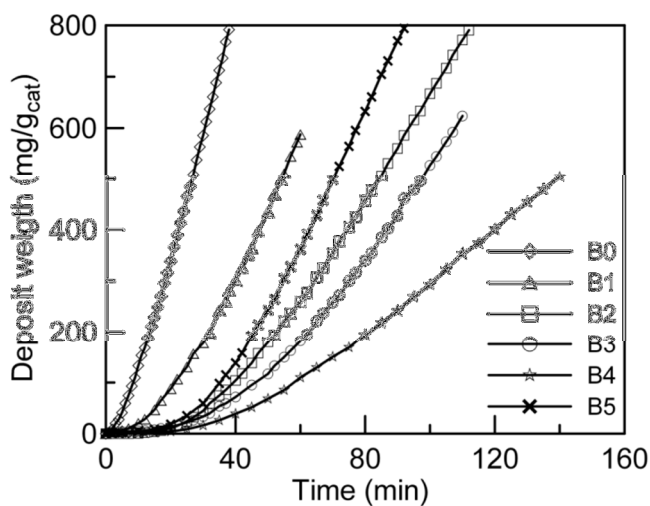
Fig. 6. Carbon deposit weight vs time in the steam reforming of n -butane. ( T = 500^{\circ}\text{C} , H_2O:C = 0.5 )
