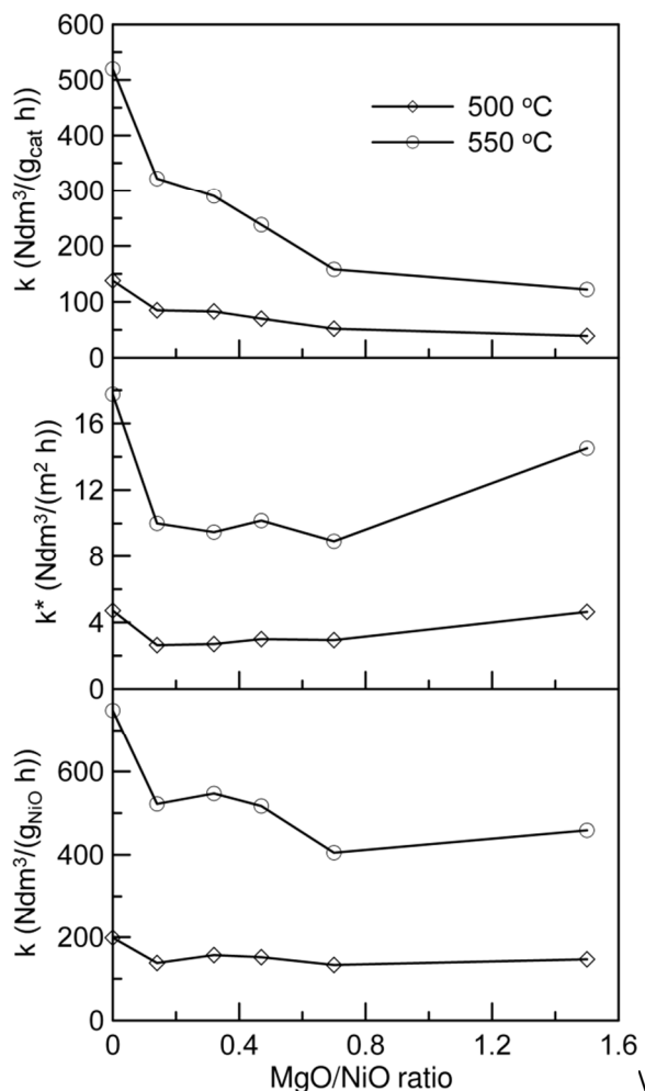
Fig. 3. The rate constants per unit of the catalyst weight, unit of the active surface area and unit of the NiO content determined at the constant \text{H}_2\text{O}:\text{CH}_4 = 2 ratio.
