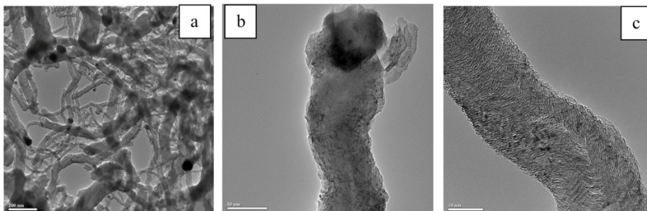
Fig. 8. Carbon deposits on B0 catalyst.
