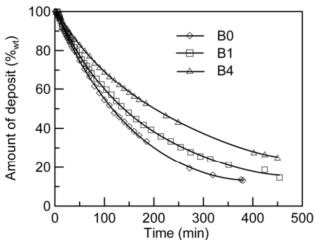
Fig. 9. Isothermal (500°C) hydrogenation of carbon deposits produced during the steam reforming of n -butane at the reagents ratio H_2O:C=0.5 .
