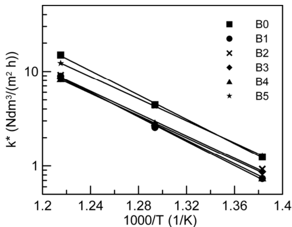
Fig. 4. The temperature dependence of the catalysts activity calculated per unit of the active surface area.
