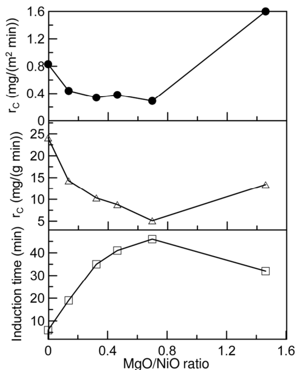
Fig. 7. Coking parameters in the steam reforming of n -butane as a function of the MgO/NiO ratio ( T = 500^\circ\text{C} , \text{H}_2\text{O}:\text{C} = 0.5 ); ( r_c – determined at 10 wt.% of the initial catalysts weight of the deposit formed).
