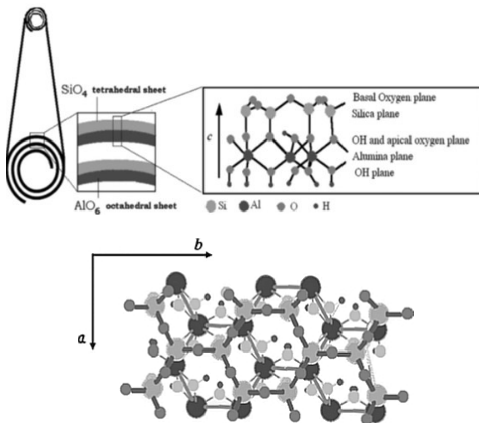
Fig. 1. The structure of halloysite [14].
